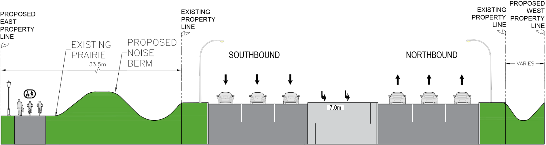
CROSS-SECTION Lagamodière Boulevard - Concept-1B & 2B
