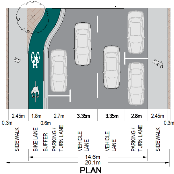
Cross-section and Plan of Westbound Goulet Street at Taché Avenue Intersection
