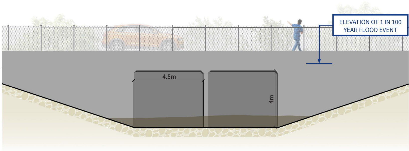
Structure Cross Section | Looking West
